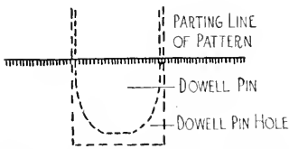
FIG. 564. WOOD DOWEL-PIN.
